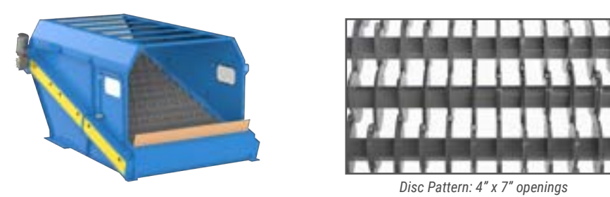
Disc Pattern: 4" x 7" openings
